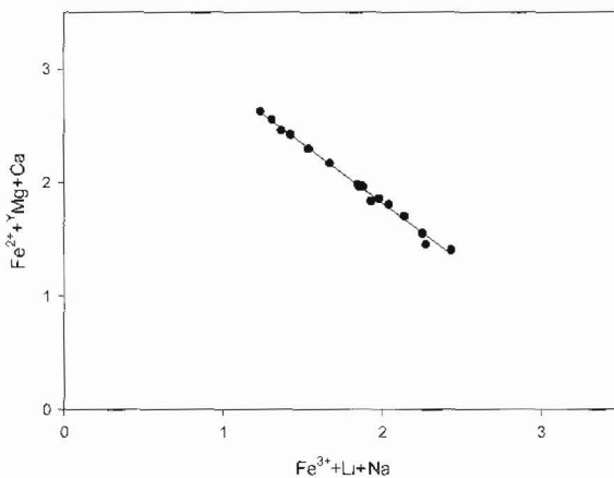
Figure 6 - The complex substitution mechanism Fe^{3+}+Na+Li \leftrightarrow Mg(Y)+Ca+Fe^{2+} , controlling the transition puvondraite \rightarrow uvite-feruvite (apfu)
