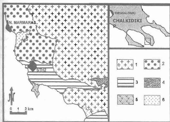
Figure 1 - Sketch map of part of the Sithonia peninsula showing sample (STH2) location. 1. Sithonia pluton; 2. Svoula flysch; 3. Chortiatis Unit; 4. Vertiskos Series; 5. Ophiolites; 6. Quaternary.
