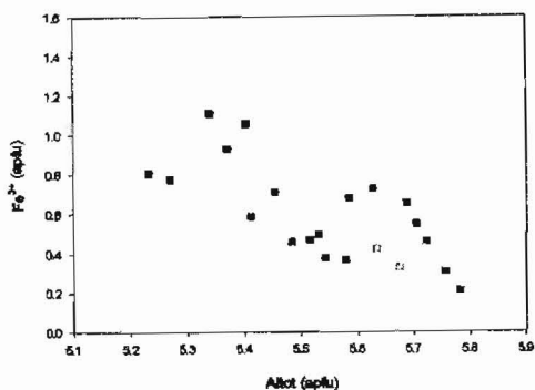
Figure 4 - Tendency of calculated Fe^{3+} vs. Al_{tot} showing a negative correlation (apfu)
