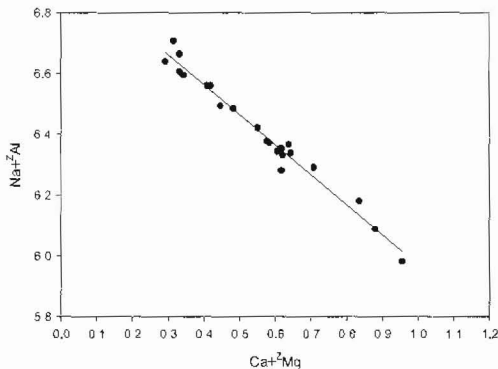
Figure 5 - Negative correlation Na+Al(Z) vs. Ca+Mg(Z) , representing the uvitic substitution (apfu)
