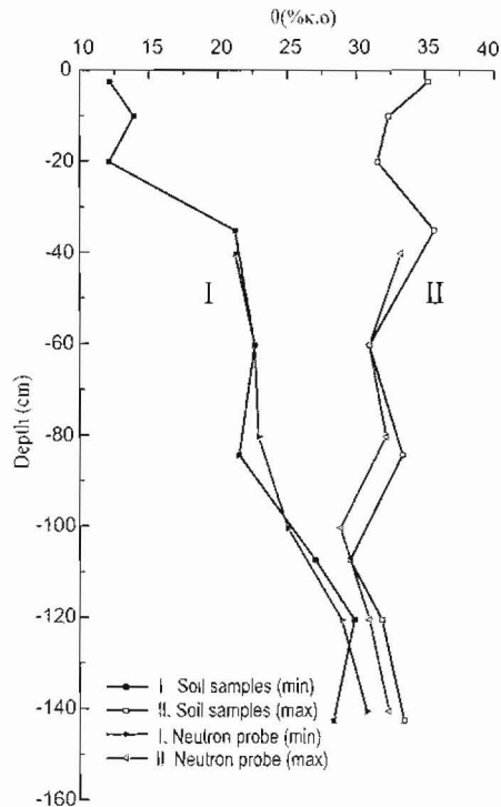
Figure 4 - Soil moisture profiles close to the minimum and maximum water contents
