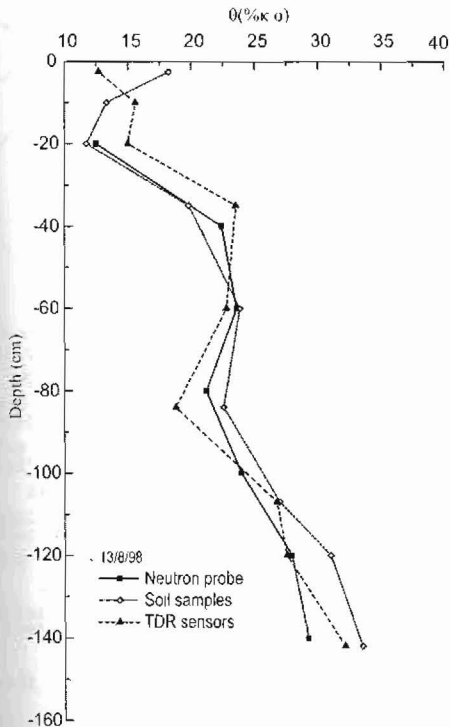
Figure 3 - Comparison of soil moisture profiles as recorded by three different methods
