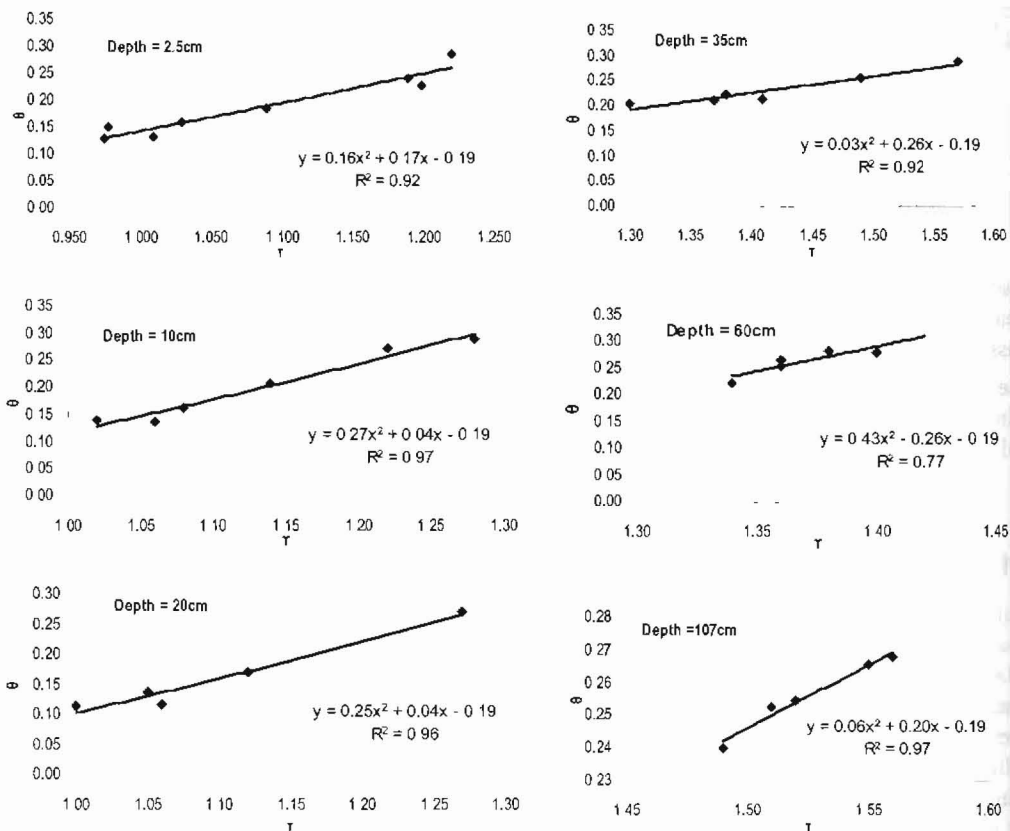
Figure 2 - Examples of TDR – sensors' calibration
