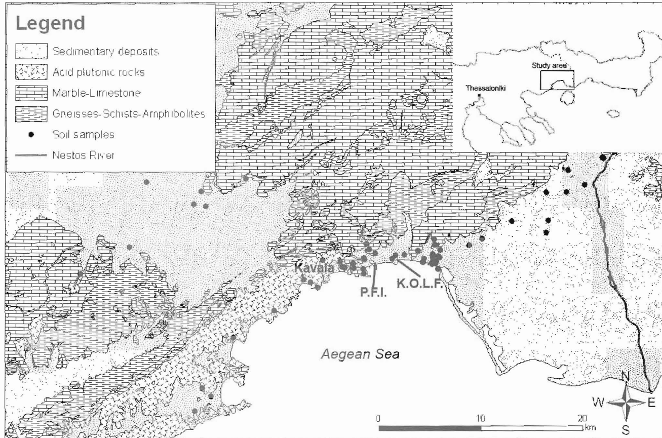
Figure 1 - Simplified geological map of the study area and location sites of the samples (modified, after IGME 1983)
