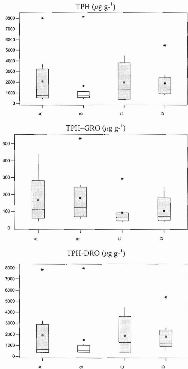
Figure 2 - Boxplots comparing concentrations of TPH, TPH-GRO and TPH-DRO at the four sampled horizons. Solid circles indicate mean values and asterisks indicate outliers
