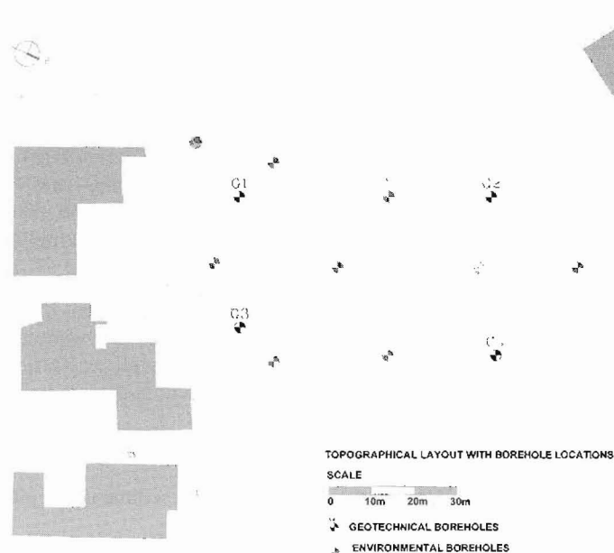
Figure 1 - Map of the sampling area showing locations of the performed geotechnical and environmental boreholes
