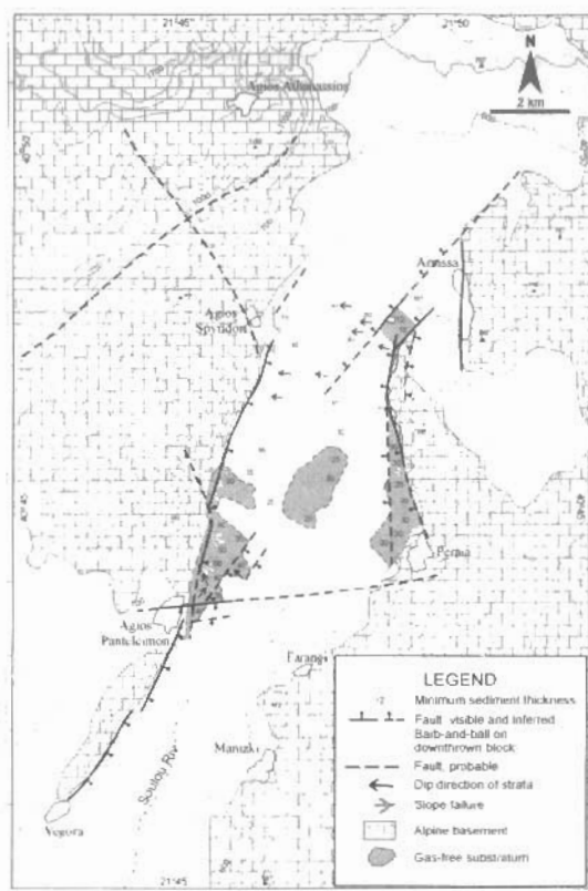
Fig. 3: Tectonic and geological map of Lake Vegoritis. Faults and geology on land after Matarangas (1981); Brunn (1982); Pavlides & Mountrakis (1987); Mercier et al (1988) and Koukouzas (1997).
