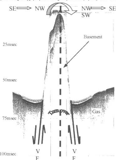
Fig. 5: BOOMER 175J seismic profile showing the steep slope formed along the Vegoritis fault at the western lakeside. For location see Fig. 3.
