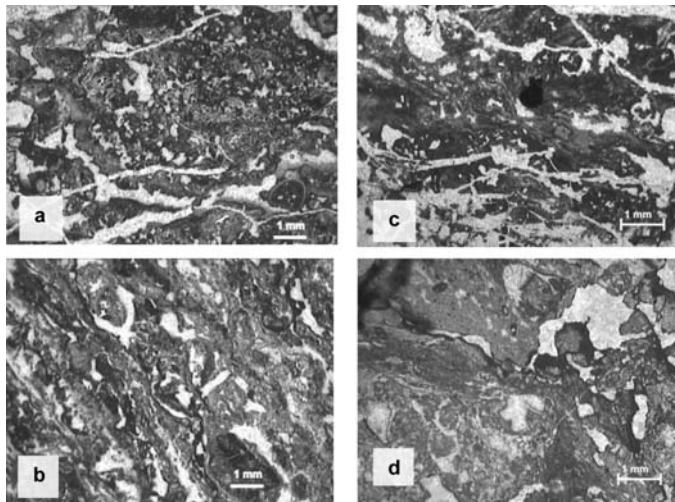
Fig. 6: Vadose environment, subaerial exposure – a. Lamina dolocrete with spar-filled interconnecting elongated cavities (Dhidyimi). b. Glaebules. Spar-filled voids and cracks (Dhidyimi). c. Microlaminated black micritic layers of pedogenic origin. Spar-filled interconnecting elongated cavities (Fokianos). d. Glaebules. Spar-filled voids and cracks (Fokianos).
