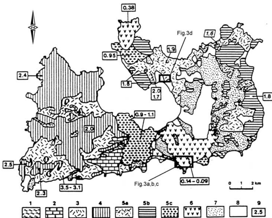
Fig. 2: Main geological units of Milos volcanic island (From Fytikas, 1976 modified). 1=Metamorphic basement; 2= Neogene sediments; 3= Basal pyroclastic series (Middle-Upper Pliocene); 4= complexes of domes and lava flows (Upper Pliocene); 5= Upper Pleistocene volcanics: pyroclastic series (5a), lava domes (5b) and Halepa and Plaka domes (5c); 6= Fyriplaka and Trachilas Rhyolitic complexes of Upper Pleistocene; 7= freatic activity products; 8= Quaternary sediments; 9= Radiometric ages from Angelier et al. (1977), Bigazzi and Radi (1981), Fytikas et al. (1976).
