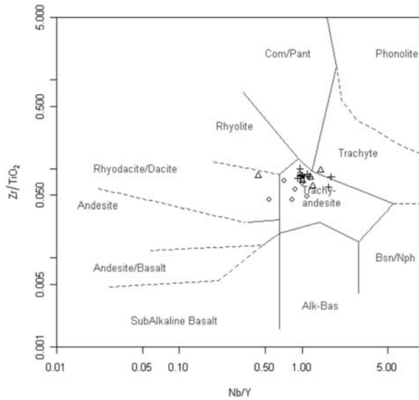
Fig. 7: Nb/Y vs. Zr/TiO 2 plot of XRF analyses of zeolitized materials from Pentalofos, Palestra and Petrota-Paleochorofa area. Diagram by Winchester and Floyd (1977). Data from Stamatakis et al. (1998).
