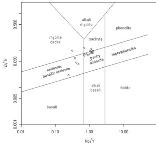
Fig. 6: Nb/Y vs. Zr/Ti plot of XRF analyses of zeolitized materials from Metaxades, Evros County, Greece. Diagram by Winchester and Floyd (1977), as modified by Pearce (1986). Data from Koutles et al. (1995).
