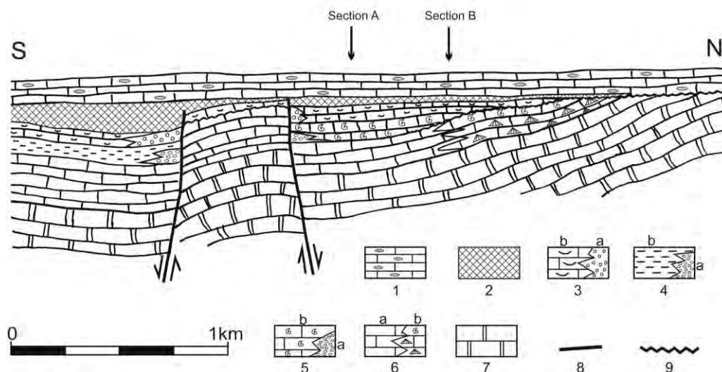
Figure 4 - Reconstruction of the deposit's architecture during Early Cretaceous; 1: Vigla limestones; 2: Upper Posidonia beds; 3: intraformational breccias (a), limestone with filaments (b); 4: intraformational breccias (a), Lower Posidonia beds (b); 5: debris flow (a), Ammonitico Rosso (b); 6: Siniais limestones (a), Louros limestones (b); 7: Pantokrator limestones; 8: fault; 9: unconformity.
