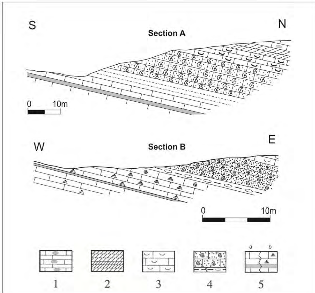
Figure 2 - Mavron Oros sections (locations are referred in Figure 1); 1: Vigla limestones; 2: Upper Posidonia beds; 3: limestone with filaments; 4: Ammonitico Rosso and base marls and/or breccias intercalations; 5: a. Siniais limestones, b. Siniais-Louros transitional limestones.
