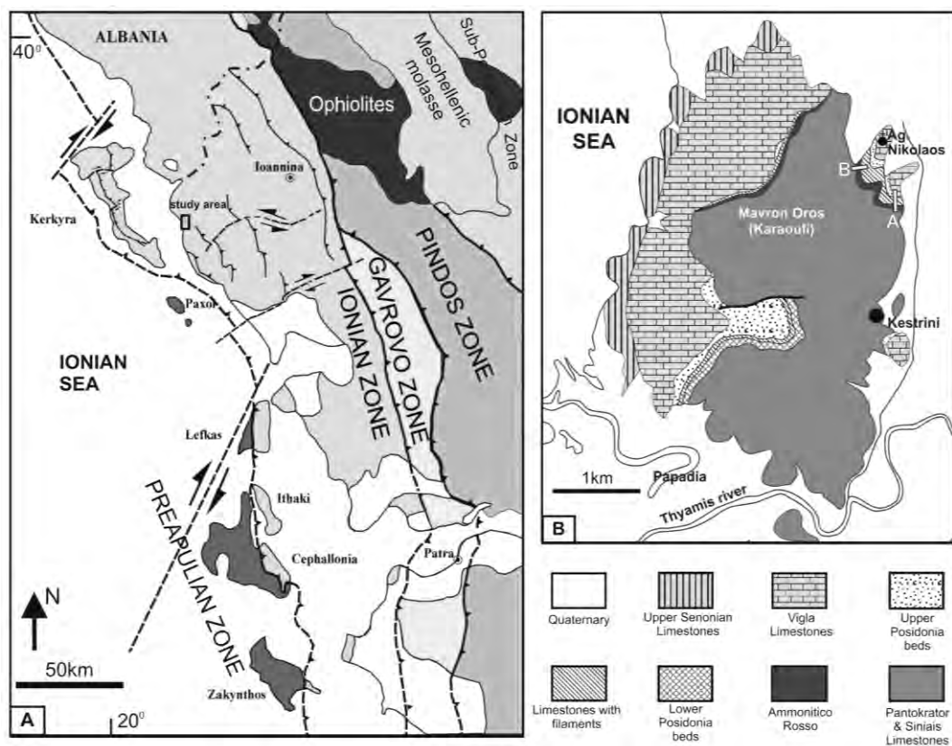
Figure 1 - A: Simplified geological map of Western Greece. B: Geological map of the study area (A and B location of the sections of Figure 2).
