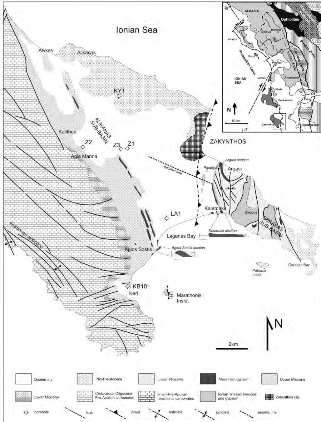
Figure 1 - Geological map of Zakynthos Island. The regional location is indicated in the inset map.
