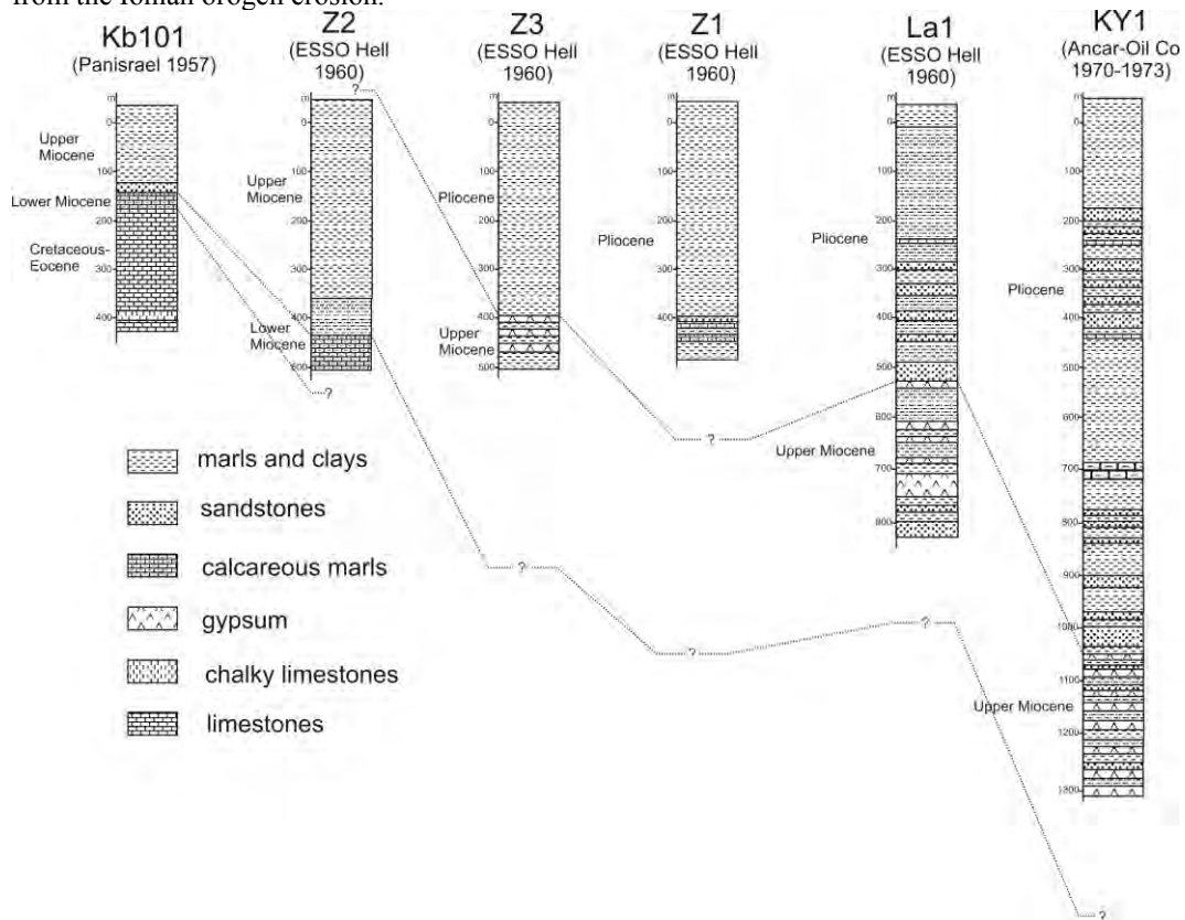
Figure 3 - Available borehole logs and correlations. Well operators are indicated.
