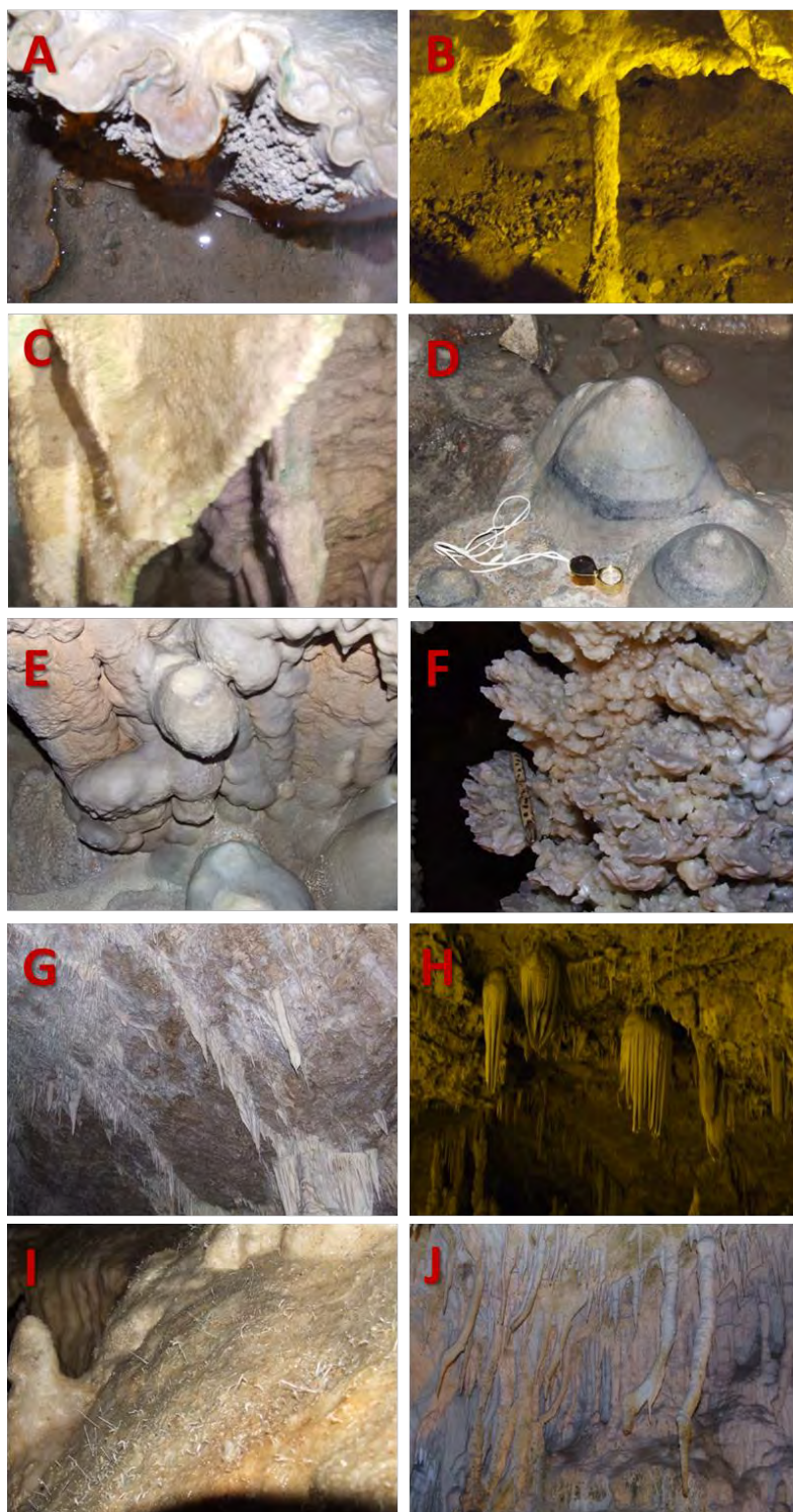
Figure 3 - Speleothem types observed in the Perama cave: A) Lotus rimstones, B) Columns, C) Draperies, D) Volcano cones, E) Punched speleothems, F) Splattermite, G) Boxwork, H) Parashute shields, I) Heligmites, J) Deflected stalactites.
