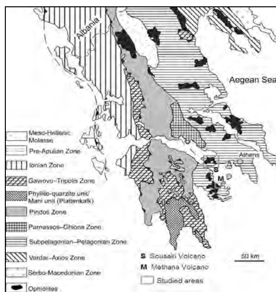
Figure 1 - Simplified geological map with the main tectonostratigraphic zones of the Hellenides and ophiolites also. The studied areas are: S (Soussaki-Geraneia) and M (Kaloni-Methana).
