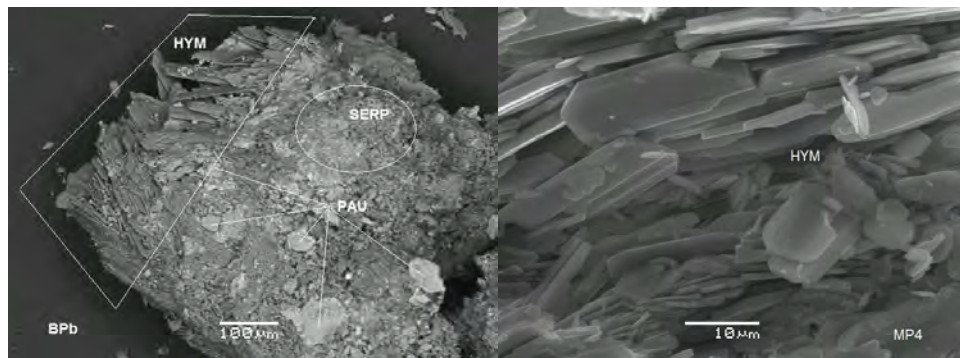
Figure 3 – SEM micrographs of Hydromagnesite (HYM) crystals (euhedral blades), in an aggregation with pyroaurite (PAU) and serpentine (SERP).
