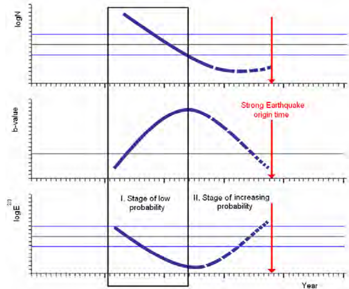
Figure 1 - Schematic representation of the temporal prognostic anomaly. Open rectangular parallelogram denotes the first, low probability stage, which is followed by an increasing probability stage. Vertical red arrow shows the earthquake origin time.
