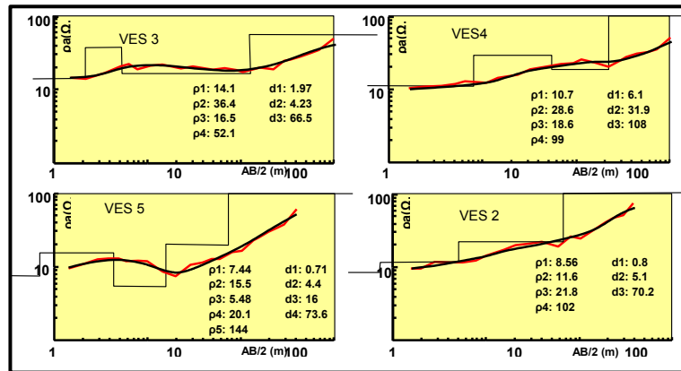
Figure 3 - Examples of Some Sounding Curves and interpretations.
