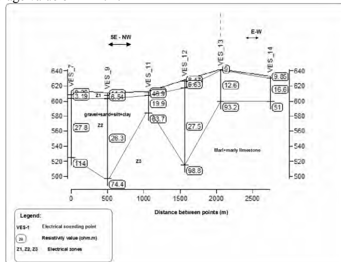
Figure 5 - Geo-electrical section along traverse 2.
