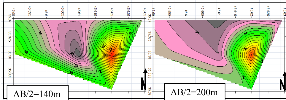
Figure 7 - Apparent resistivity map for AB/2 equal to 140 m and 200 m.
