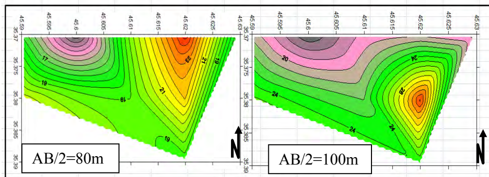
Figure 6 - Apparent resistivity map for AB/2 equal to 80 and 100m.
