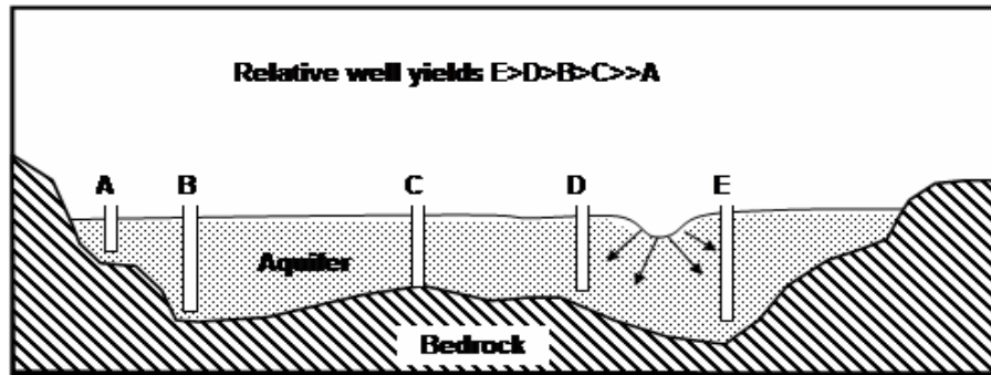
Figure 8 - Hypothetical cross section of a valley showing the effects of aquifer thickness and hydrogeologic boundaries on well yield (Davis and DeWiest, 1976).
