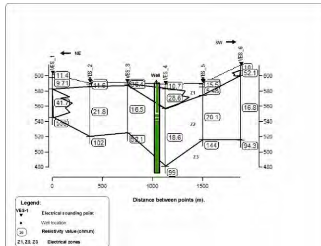
Figure 4 - Geo-electrical section along traverse 1.
