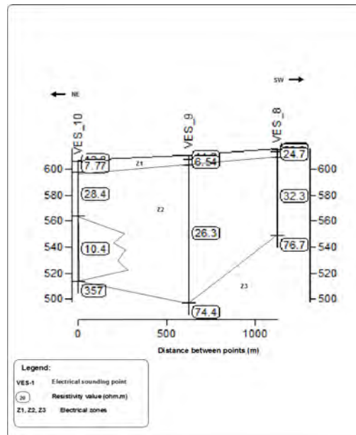
Figure 6 - Geo-electrical section along traverse 3.
