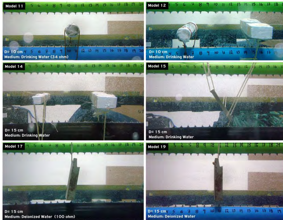
Figure 7 - Targets for detection embedded inside water (void cylinder, polystyrene, metal plates).
