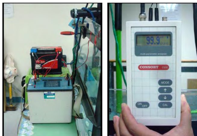
Figure 6 – (left) “Iris” instrument for acquiring electrical data, (right) “Consort” a conductivity meter for measuring medium inside tank.
