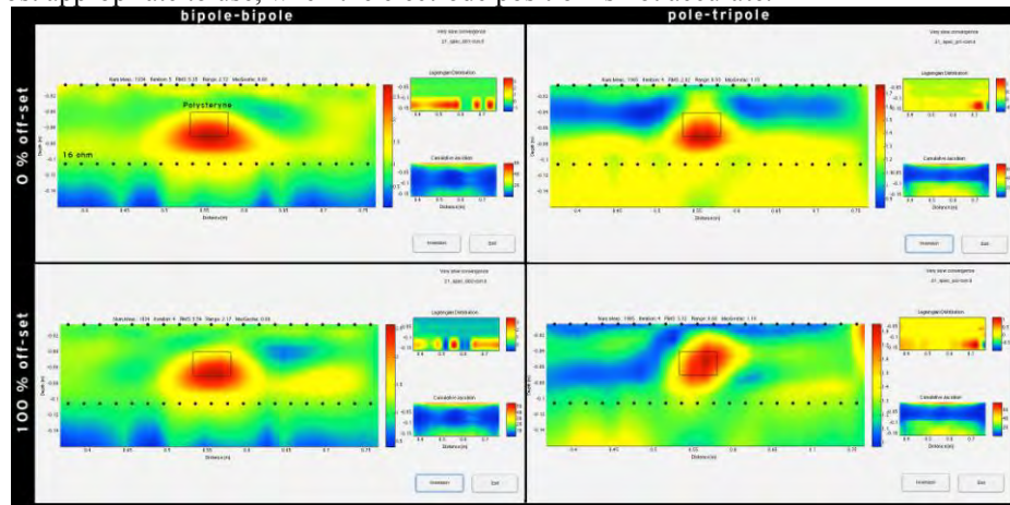
Figure 12 – Inversion results with 0% (top row) and 100% (bottom row) electrode displacement for protocol bb (left column) and pt (right column).
