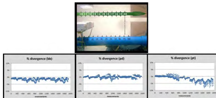
Figure 11 – Offset calculated with electrode displacement (top), % divergence occurred (bottom).
