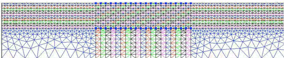
Figure 1 – Mesh (created by FEM) used using surface to tunnel measurements.
