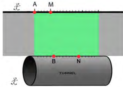
Figure 2 – Application of surface-to-tunnel arrays (A, B current electrodes, M, N potential electrodes).
