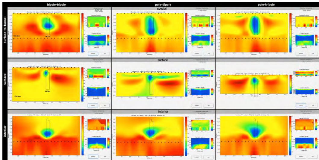
Figure 8 - Inversion results using conductive target inside water.
