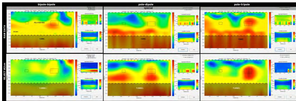
Figure 10 – Inversion results depicting target above a tunnel raw data (top row) and corrected data (bottom row).
