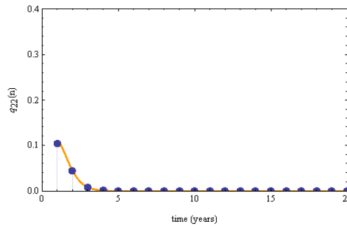
Figure 8 - Kernel probabilities q_{22}(n) , of the discrete Weibull distribution.
