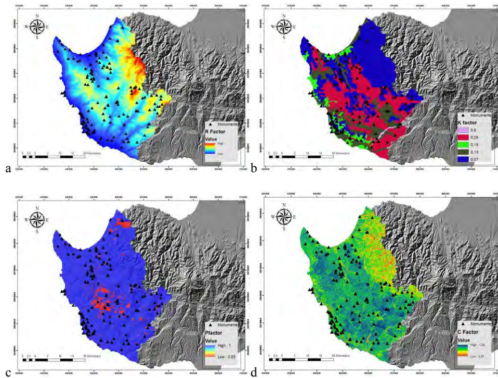
Figure 4 - P factor (a). K factor (b). R factor (c). RUSLE model of the study area (d).
