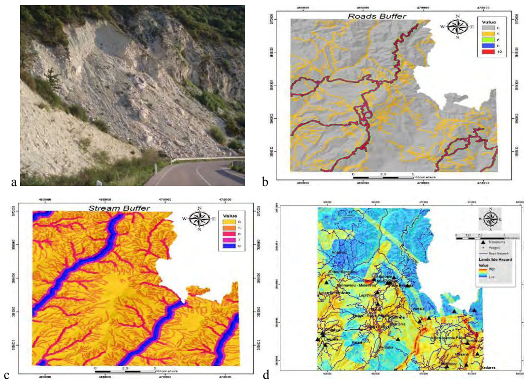
Figure 5 - Rock slide in chalk across a roadcut (a). Road buffer (b). Stream buffer (c). Landslide hazard assessment map (d).
