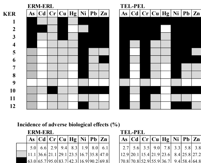
Figure 2 - Evaluation of aquatic life impairment due to the heavy metal load of the study area sediments using the marine ERM/ERL and TEL/PEL Guidelines.
