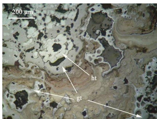
Figure 3 - Concentric shells of goethite alters progressively to hematite. (gt:goethite, ht:hematite) Reflected light, // Nicols.
