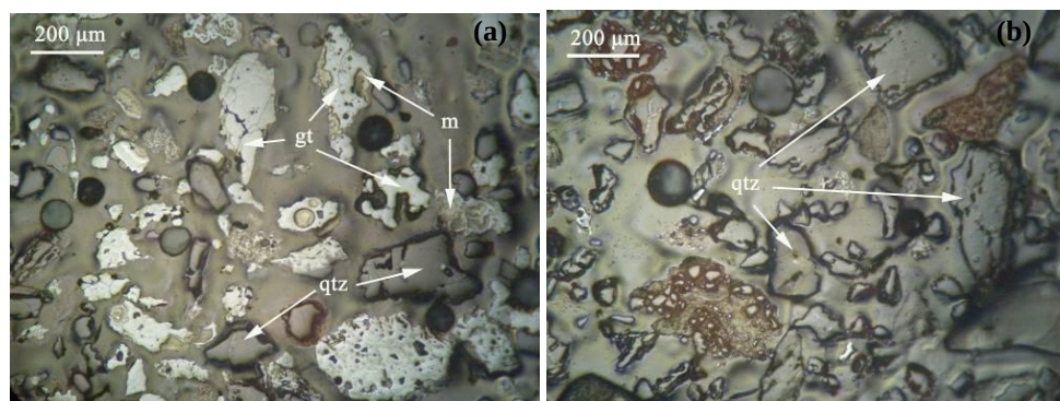
Figure 5 - Goethite grains and matrix partially liberated. Quartz is also present. (size fraction -0.250+0.063 mm). a. Sink b. Float (gt: goethite, qtz: quartz, m: matrix). Reflected light, // Nicols.
