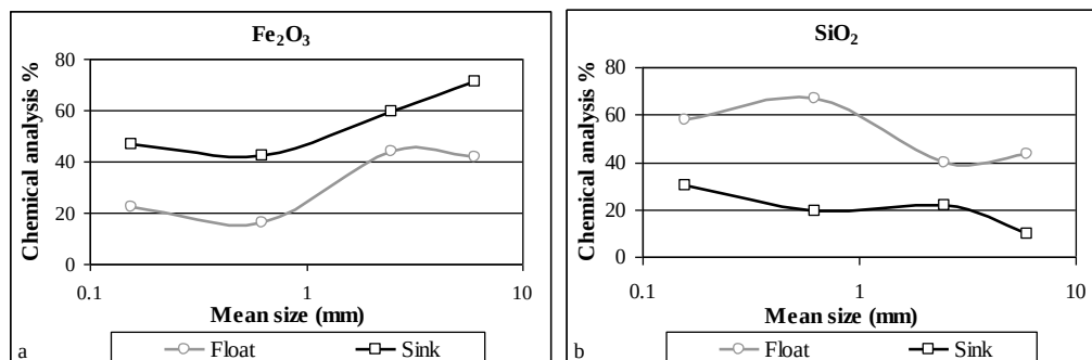
Figure 4 - \text{Fe}_2\text{O}_3 (%wt) (a) and \text{SiO}_2 (%wt) (b) contents of the products obtained from the gravimetric separation.
