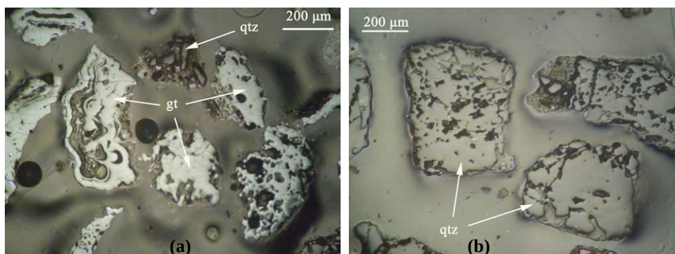
Figure 7 - Goethite grains with traces of quartz of size fraction -1+0.250 mm. a. Magnetic product 1 b. Non magnetic product. (gt: goethite, qtz: quartz). Reflected light, //Nicols.
