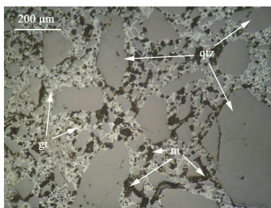
Figure 2 - Goethite replacing progressively the matrix between the grains of phyllite-quartzite. (gt:goethite, qtz: quartz, m: matrix). Reflected light, // Nicols.
