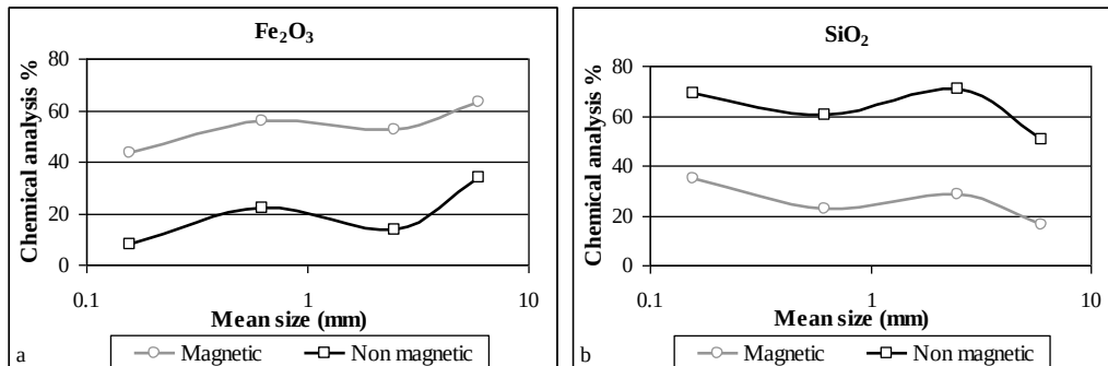
Figure 6 - Fe 2 O 3 (%wt) (a) and SiO 2 (%wt) (b) content of magnetic separation products.
