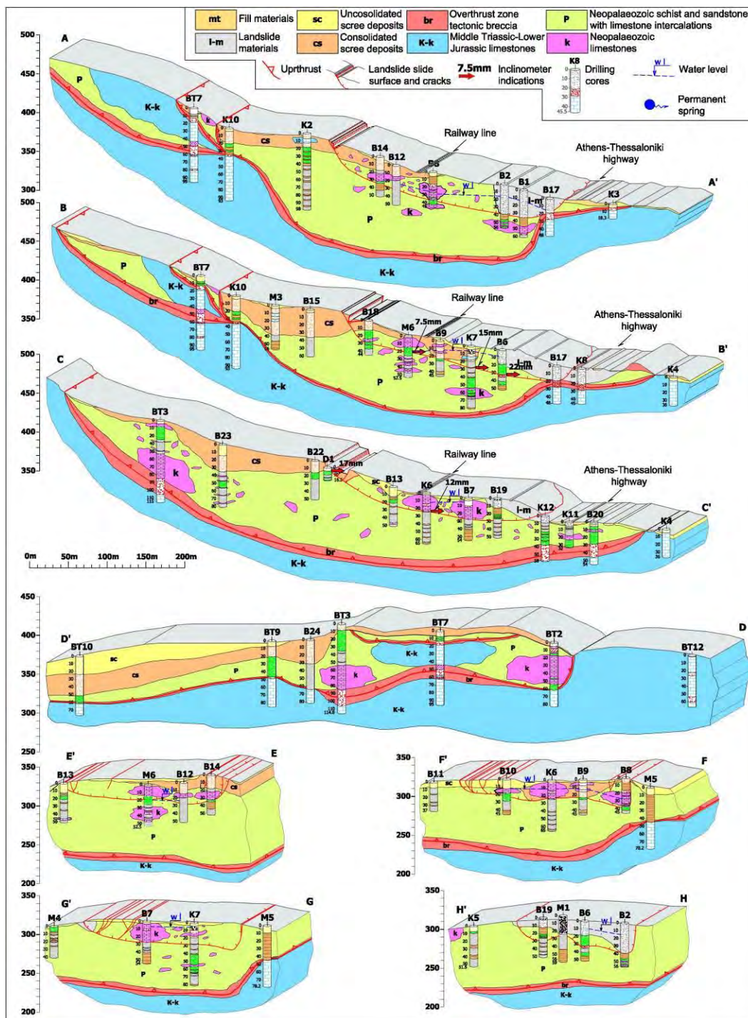
Figure 3 - Geological cross-section of Malakasa landslide.
