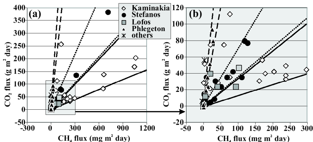
Figure 2 - \text{CH}_4 vs. \text{CO}_2 fluxes. The right graph is the enlargement of the left one. The black lines represent the range of \text{CO}_2/\text{CH}_4 concentration ratios in the Kaminakia fumaroles, the stippled line that of the Stefanos fumaroles and the dashed lines that of the Phlegeton fumaroles.
