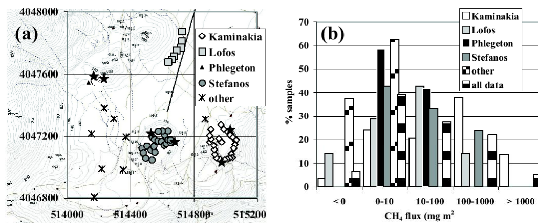
Figure 1 - (a) study area with CH 4 flux measurements points and sampled gas manifestations (stars). (b) Percent frequency distribution of CH 4 flux values.
