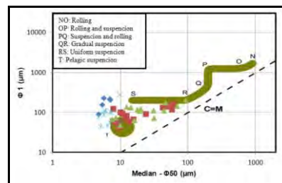
Figure 11 - Diagram of Passega (1957) 1964) for the determination of the depositional environment.
