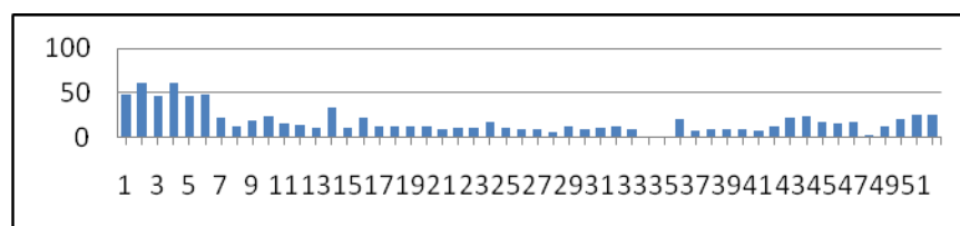
Figure 13 - The content of CaCO 3 in studied deposits.
