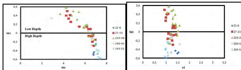
Figure 9 - Diagram of Valia and Cameron (1979), showing the depositional depth (Sk1=asymmetry, Mz=mean and σ1= deviation).
