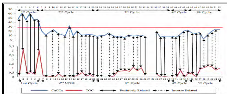
Figure 14 - Correlation of \text{CaCO}_3 and TOC contents within studied deposits.
