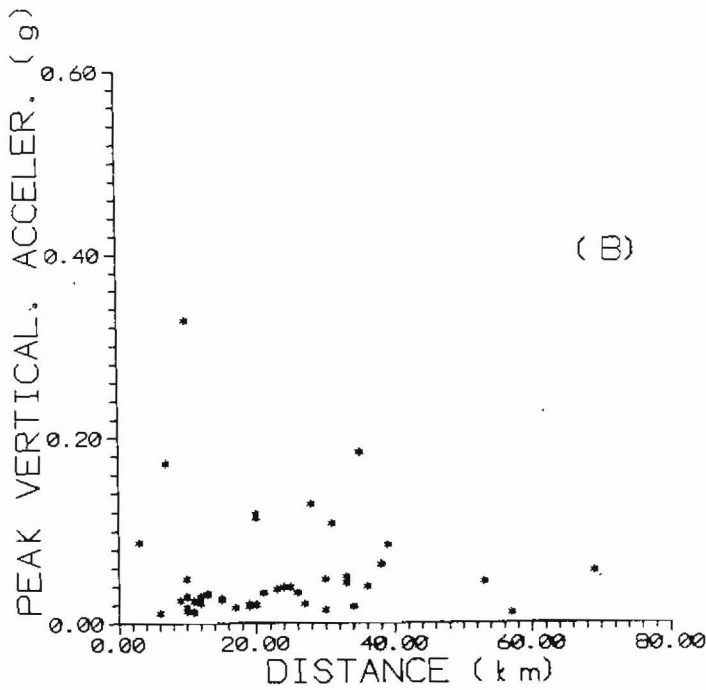
Fig.4. The peak horizontal acceleration (A) and the peak vertical acceleration (B) versus distance.
