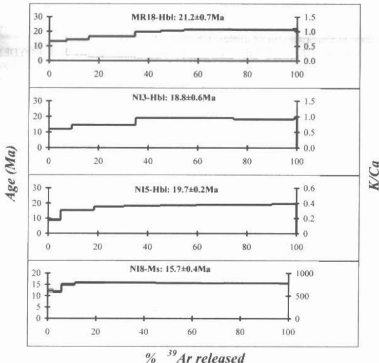
Fig. 3b: Graphical representation of the results obtained by the incremental heating technique of hornblende and muscovite separates from the Pangeon granitoids.
