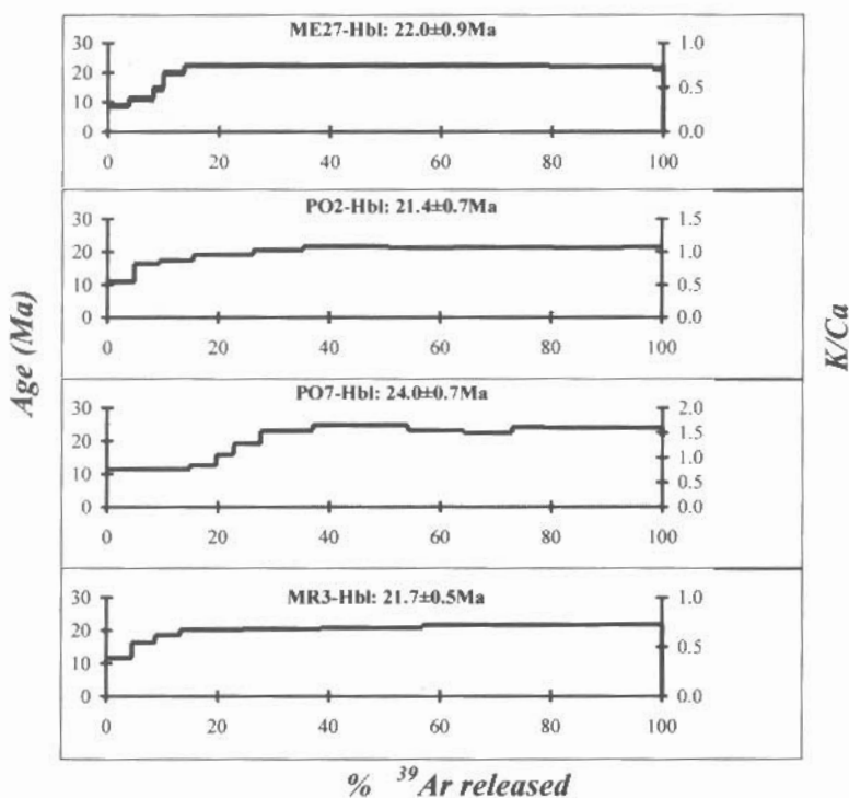
Fig. 3a: Graphical representation of the results obtained by the incremental heating technique of hornblende separates from the Pangeon granitoids (continued)
