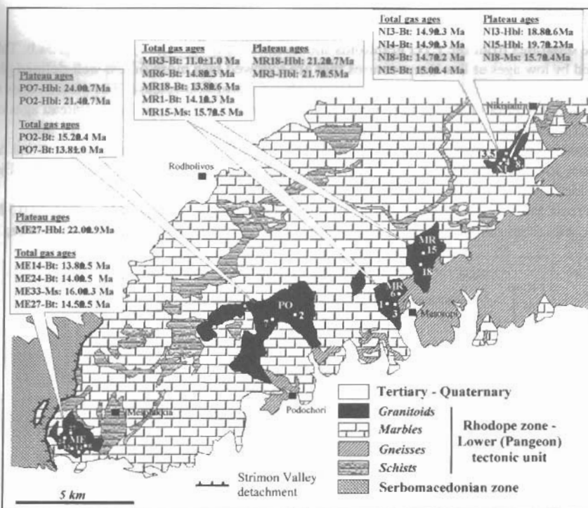
Fig. 2: Simplified geological map (after Schenck, 1970) of the Pangeon granitoids showing the major lithologic types of the sampling area, the sample name and location and the Ar/Ar-ages obtained from Bt (biotite), Hbl (hornblende) and Ms (muscovite) separates.
