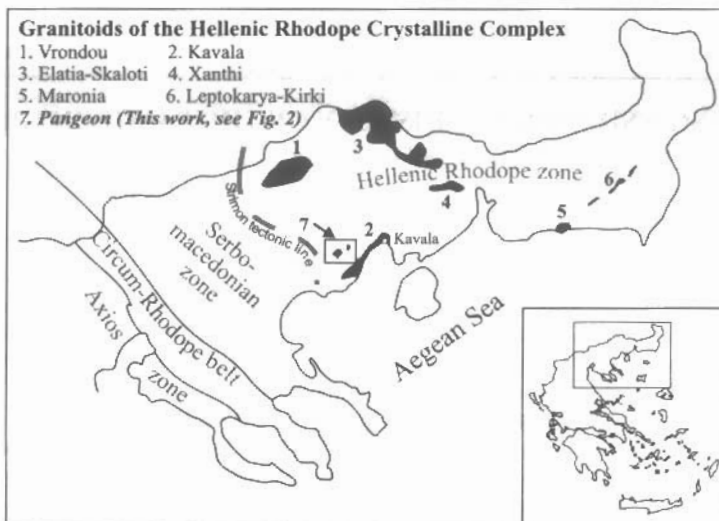
Fig. 1: Simplified geologic map of the Hellenic Rhodope Crystalline Complex showing the distribution and names of the main occurrences of granitoid rocks.
